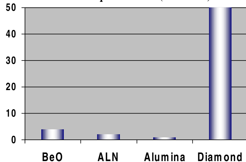
Power Rating in Watts of 50 square mils (1.27mm)
